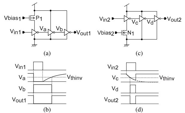
Fig. 6 Delay and inversion circuits and their timing diagrams: (a),(b) delay & inv 1 , (c),(d) delay & inv 2 .
