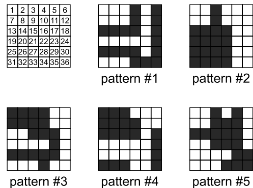
Fig. 8 Stored patterns.
