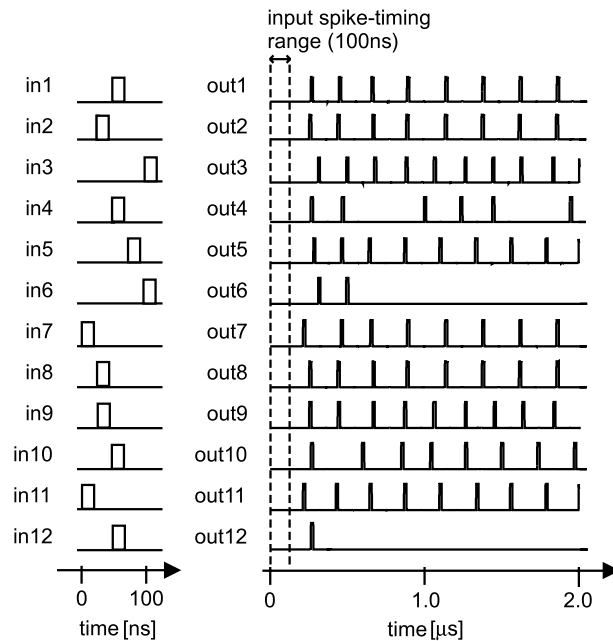
Fig. 10 Simulation result without GEU .
