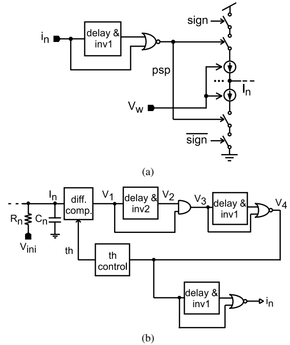
Fig. 4 Spiking neuron circuits: (a) synapse and (b) neuron.
