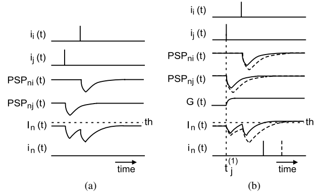
Fig. 2 Examples of input/output spike trains and neuronal internal potentials without (a) and with (b) GEU.
