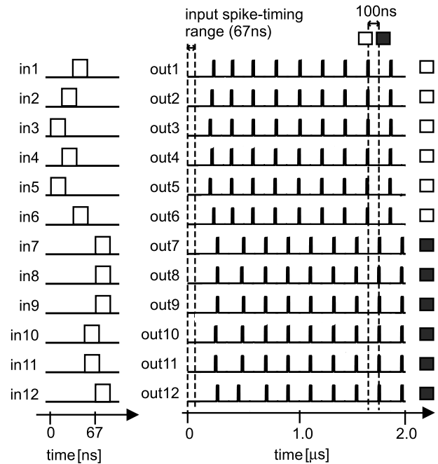
Fig. 16 Simulation result when the input spike-timing range is smaller than half of the transmission delay time.
