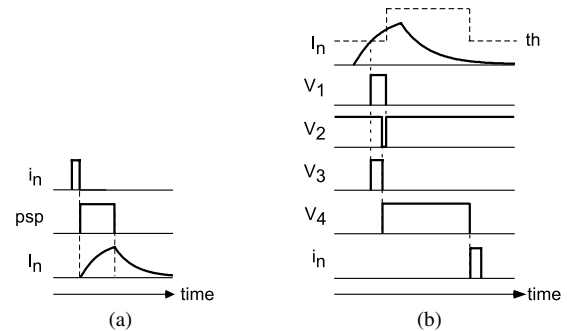
Fig. 5 Timing diagrams of spiking neuron circuits: (a) synapse and (b) neuron.
