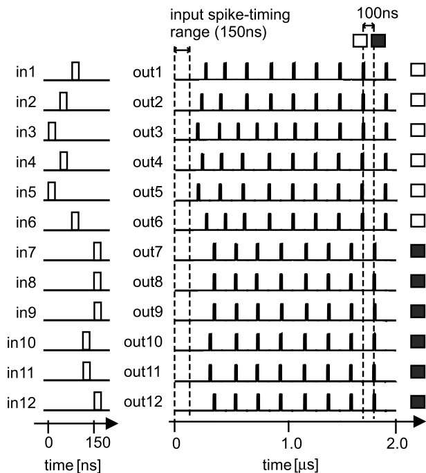
Fig. 17 Simulation result when the input spike-timing range is larger than half of the transmission delay time.
