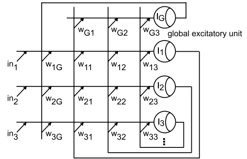
Fig. 3 Spiking feedback network model with GEU .
