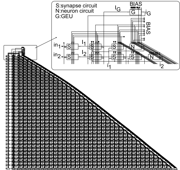
Fig. 7 Block diagram of a spiking feedback neural network circuit with GEU .
