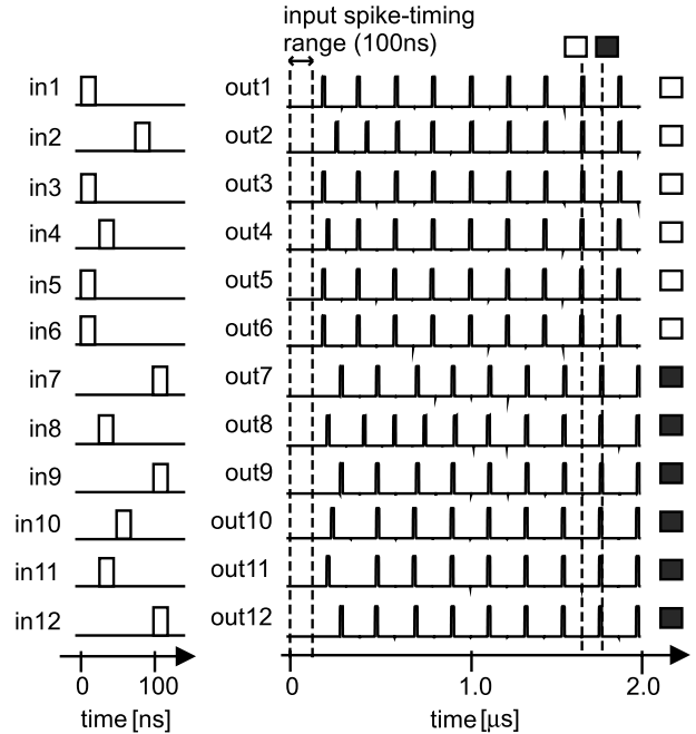
Fig. 15 Simulation result with GEU to stored pattern #6.
