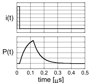
Fig. 9 Typical time course of PSP for input i(t) .
