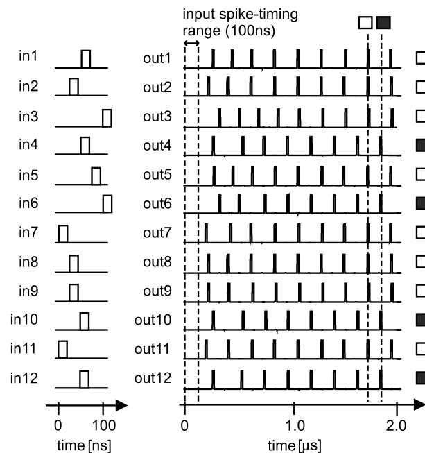
Fig. 11 Simulation result with GEU .
