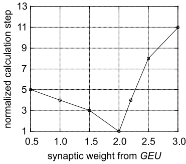
Fig. 12 Relationship between the synaptic weight from GEU and the normalized calculation steps required for recalling.
